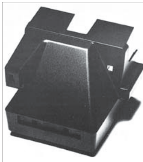
Photo-textured body for Polaroid instant camera. Mould material: Stavax ESR.
